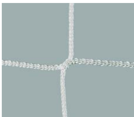
No. 200: White, knotless high tenacity polypropylene, approx. 2.3 mm.
